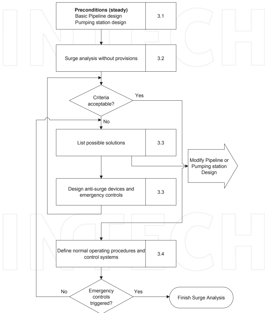
Figure 2. Integrated design for pressure transients and controls.
