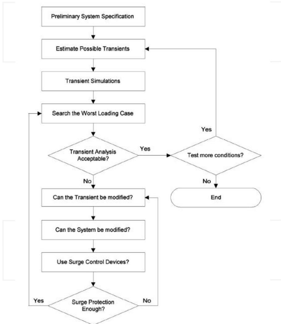
Figure 1. Pressure Transient design (Jung and Karney 2009).
